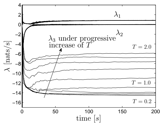
(b) CLDYN method.
