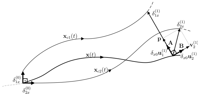
Fig. 1 Illustration of a typical CLDYN iteration. \delta_{1x}^{(0)} and \delta_{2x}^{(0)} are the initial difference state vectors given by \delta_{x0}\{\mathbf{e}_1, \mathbf{e}_2\} . \mathbf{p} is the projection of \delta_{2x}^{(1)} in \delta_{1x}^{(1)} used to obtain \mathbf{v}_2 vector. A and B represent the initial conditions for the next iteration of the procedure. The value of \delta_{x0} was exaggerated here for the sake of the illustration.
