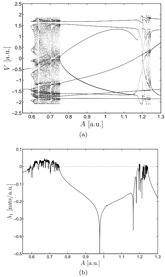
Fig. 5 Figure 5(a) is the estroboscopic map taking the amplitude A [a.u.] as control parameter of the FitzHugh-Nagumo model; V [a.u.] is the state variable membrane potential. Figure 5(b) represents the largest Lyapunov exponent associated to the respective control parameter.
